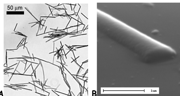
Figure 2. (A) Optical micrograph of the SU-8 microrod particles dispersed in water. (B) SEM image of a single SU-8 microrod partially embedded on PDMS after being picked up from the oil-water surface with the GTT. 8 The visible part of the microrod has initially been in contact with the aqueous phase, while the part embedded in the PDMS has been in contact with the oil.
